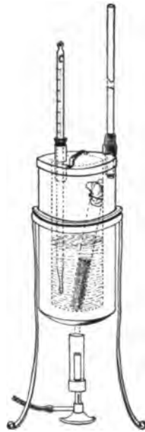
FIG. 140.—Benzole bath.
